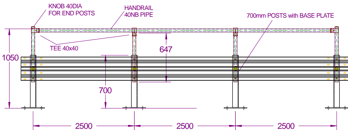
General Handrail Layout
